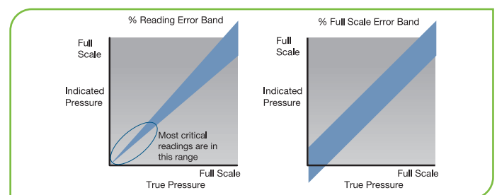
Figure 1 - Comparison of MKS repeatability expressed as percent of Reading transducer versus other percent of Full Scale transducers.
