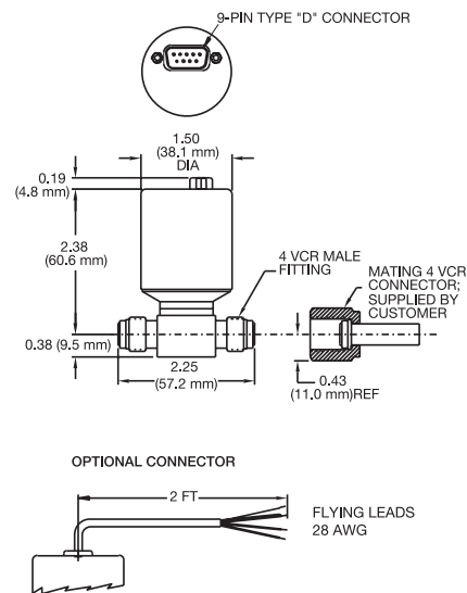
Output Connections
