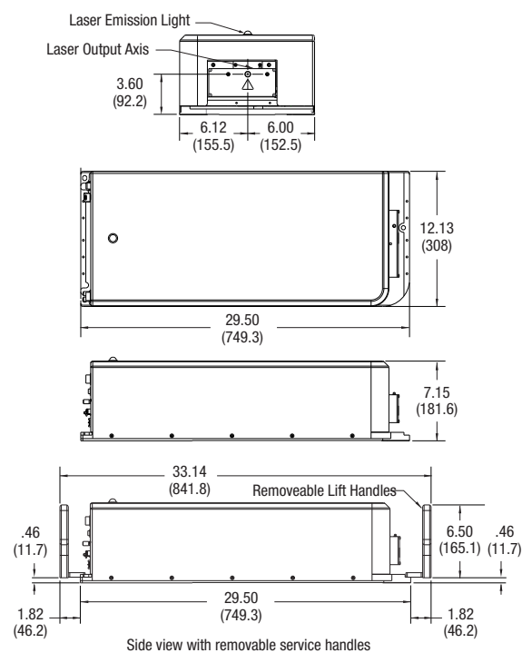
IceFyre UV50 Laser Dimensions
