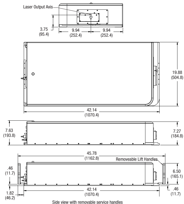
IceFyre IR50 Laser Dimensions
