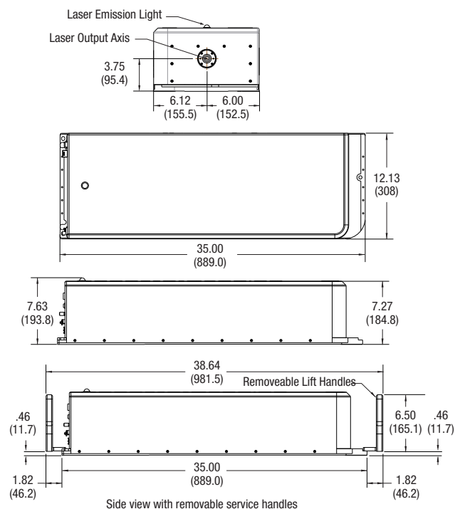
IceFyre UV30 and GR50 Laser Dimensions
