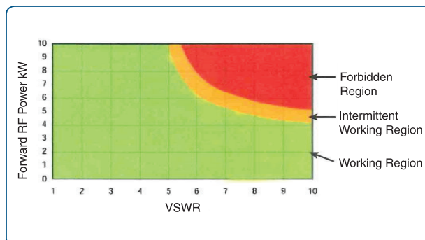
Figure 1 — Operating Graph
