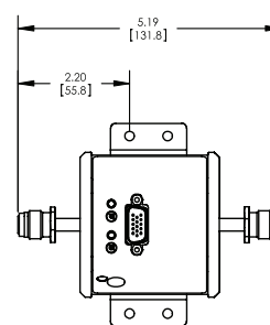
MALE VCR FITTING CODE "CB"
