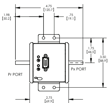
1/4" TUBE STUB FITTING CODE "BB"
